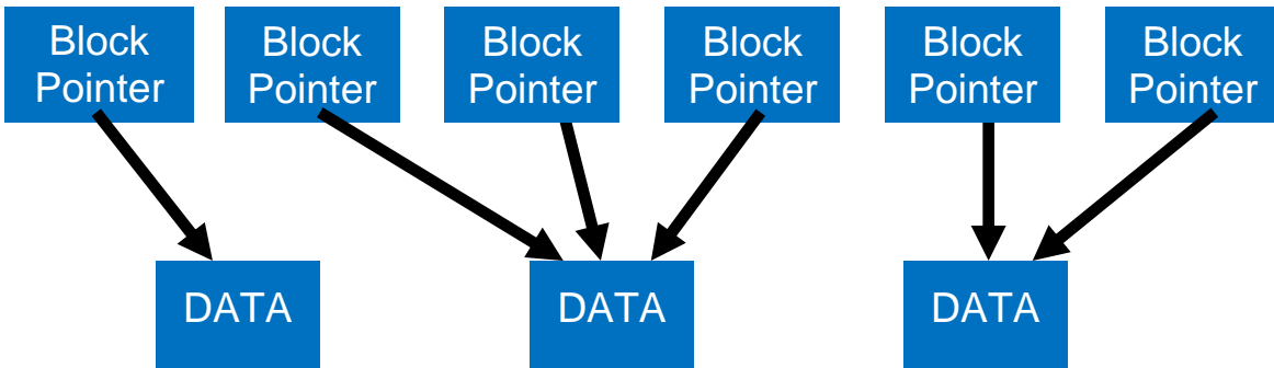
Figure 2) Data structure in a deduplicated FlexVol volume or data constituent.
